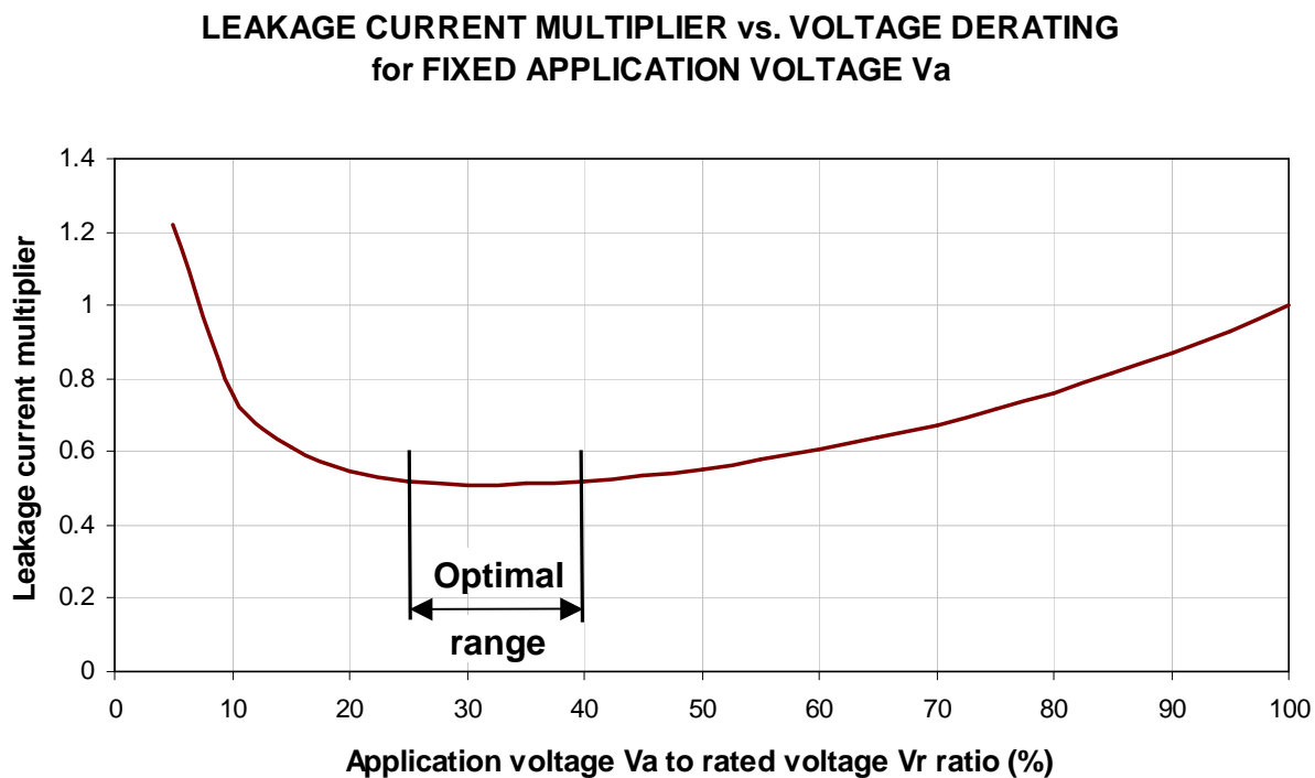
Figure 6: Graph of maximal actual DCL vs voltage derating
