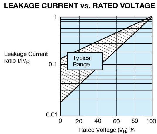
Figure 4: Effect of voltage derating on DCL
