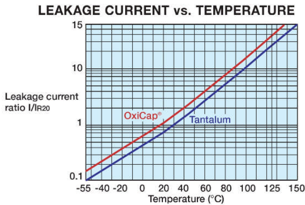
Figure 3: Temperature dependence of DCL
