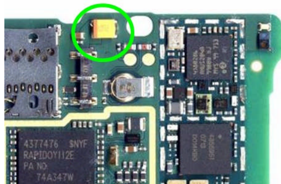
Figure 1: Battery circuit tantalum capacitor in handheld device
