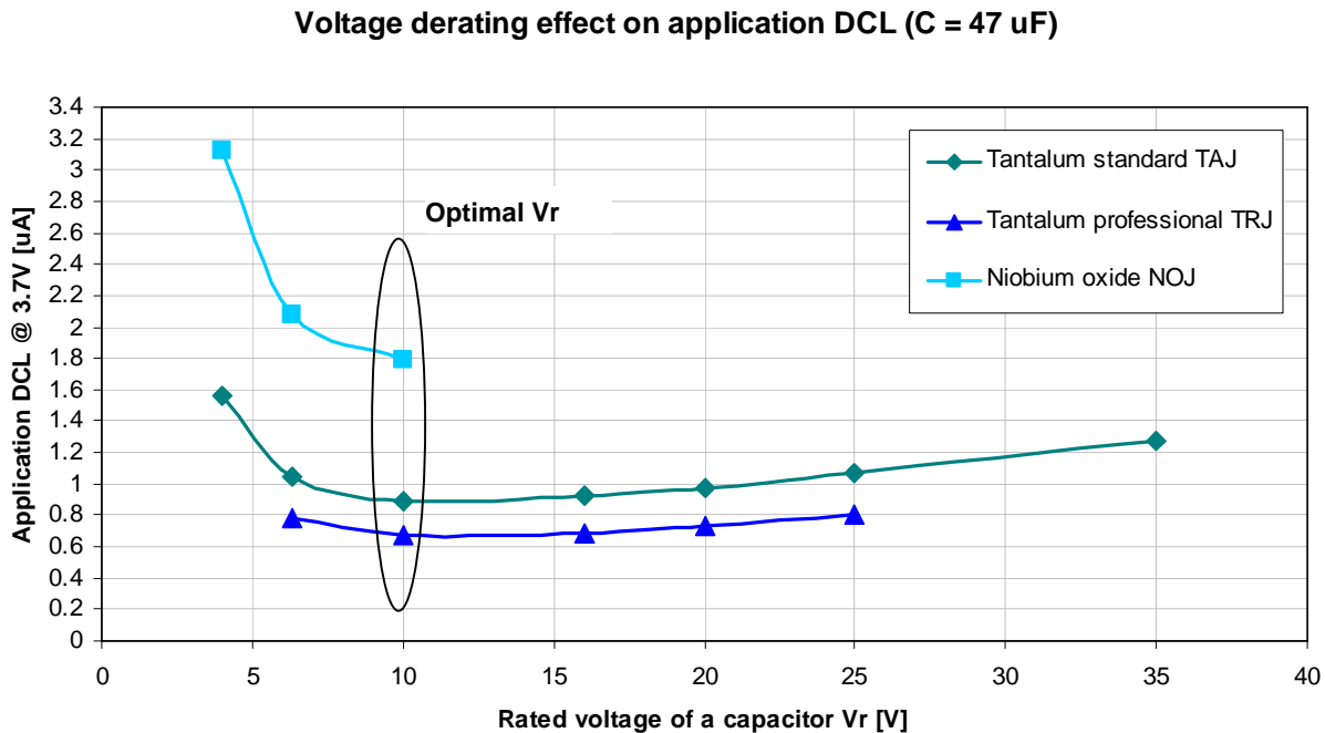
Figure 7: Benchmark of maximal actual DCL of different capacitor series
