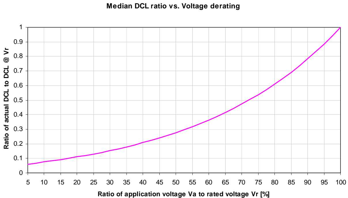
Figure 5: Median curve of typical range of DCL vs Voltage derating from Figure 4
